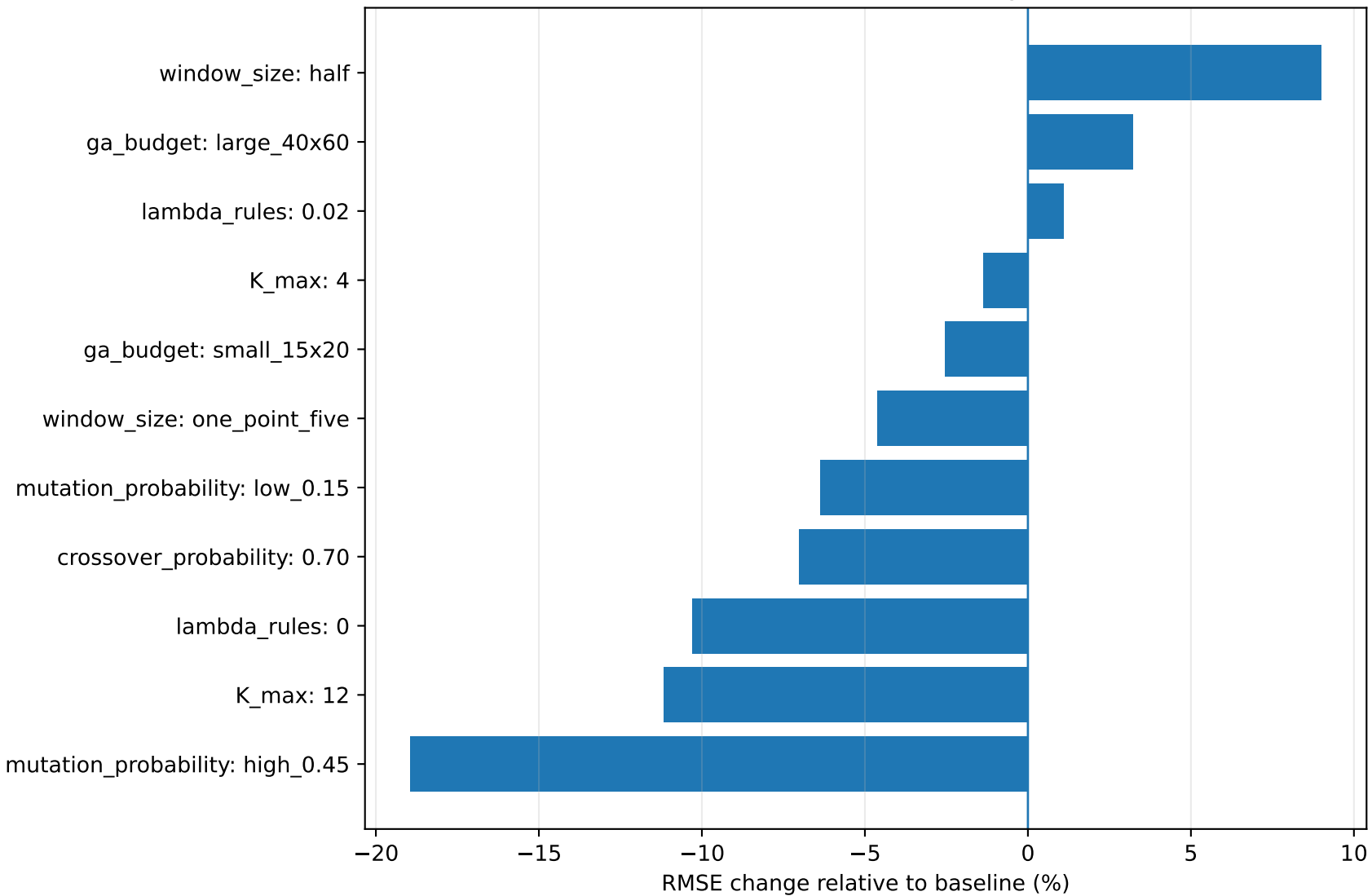
NFGA-LINEAR one-factor sensitivity — Cholera
