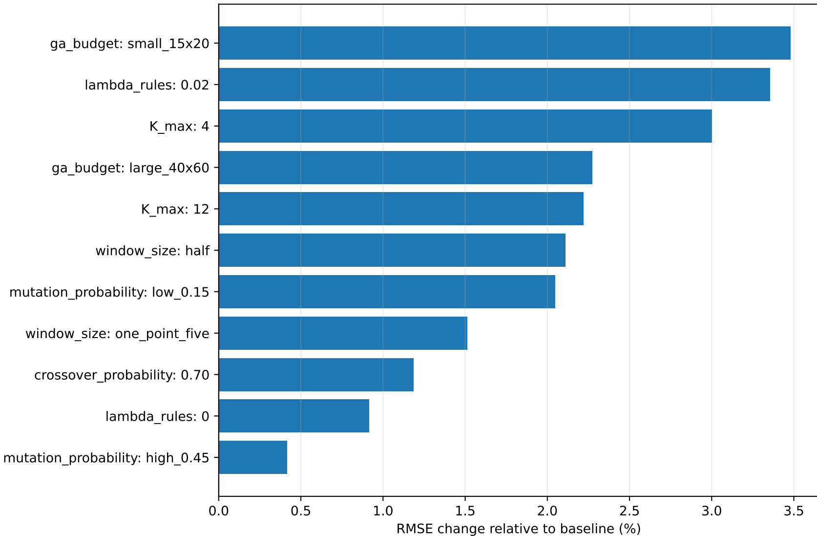
NFGA-LINEAR one-factor sensitivity — Ilinet
