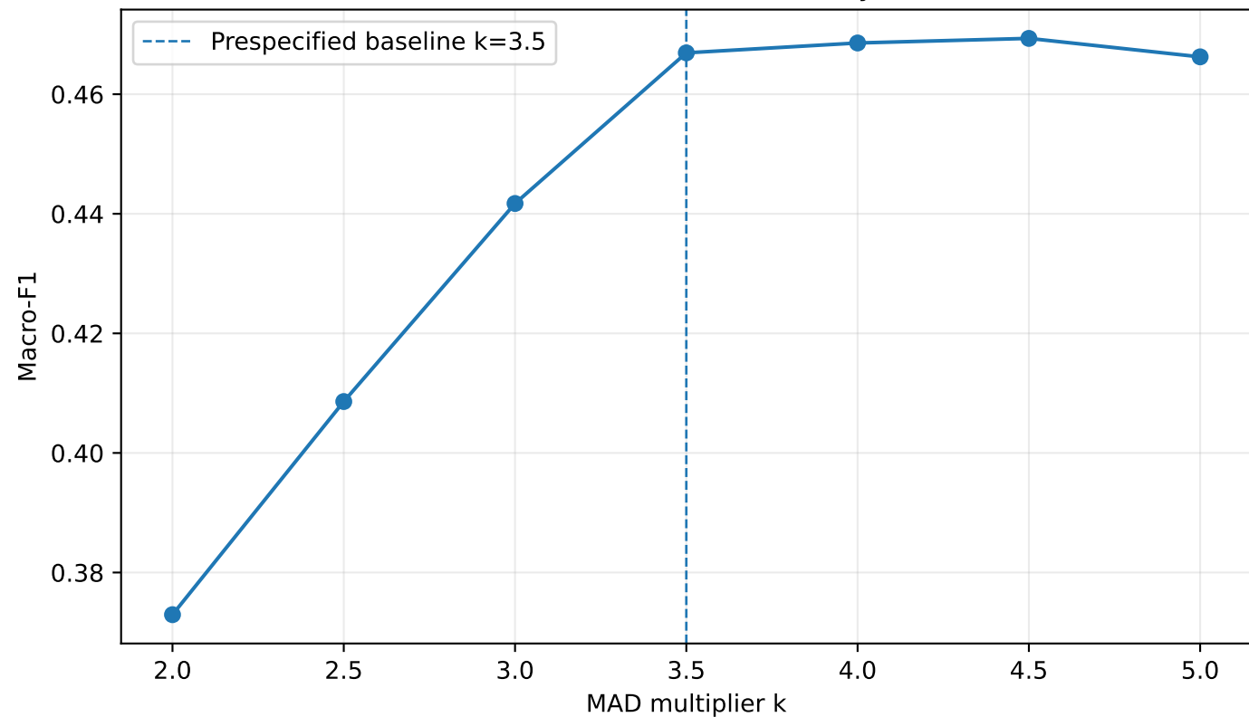
NFGA-LINEAR threshold sensitivity — llinet
