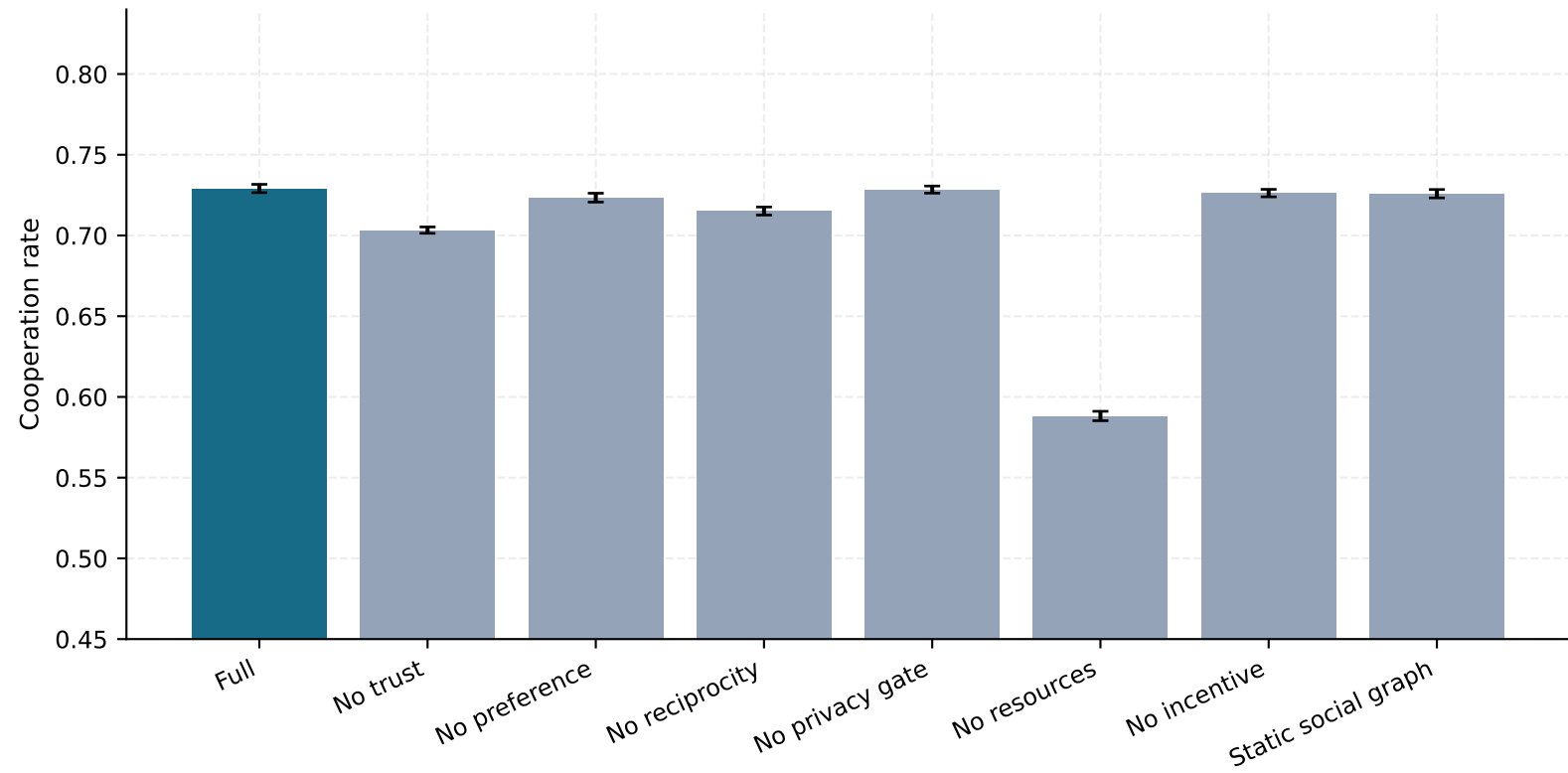
Behavioral ablation at high load (50 paired seeds)
