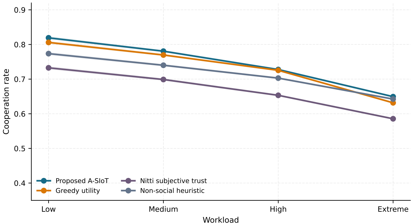
Benign cooperation across paired workloads (100 seeds)
