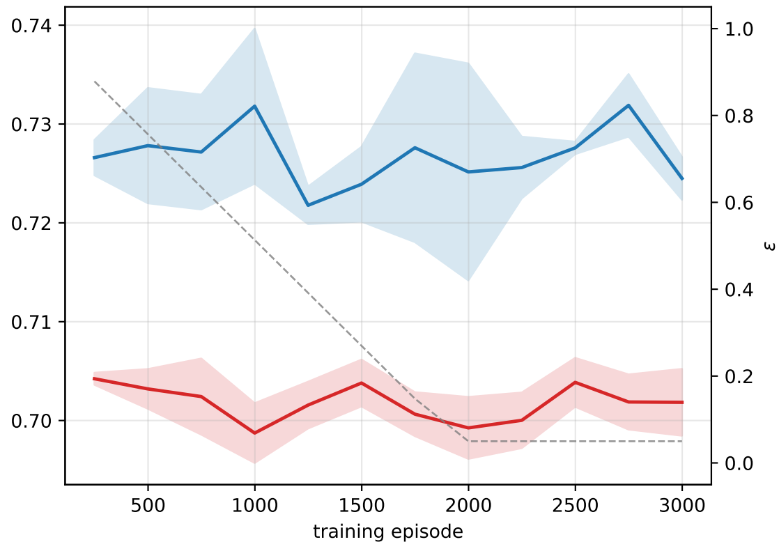
Frozen evaluation cooperation rate
