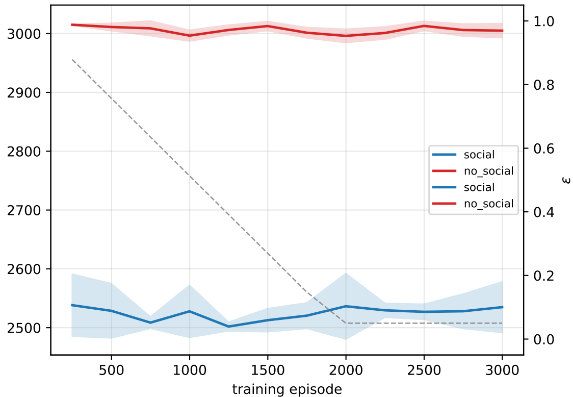
Frozen evaluation reward (sum over 500 steps)
