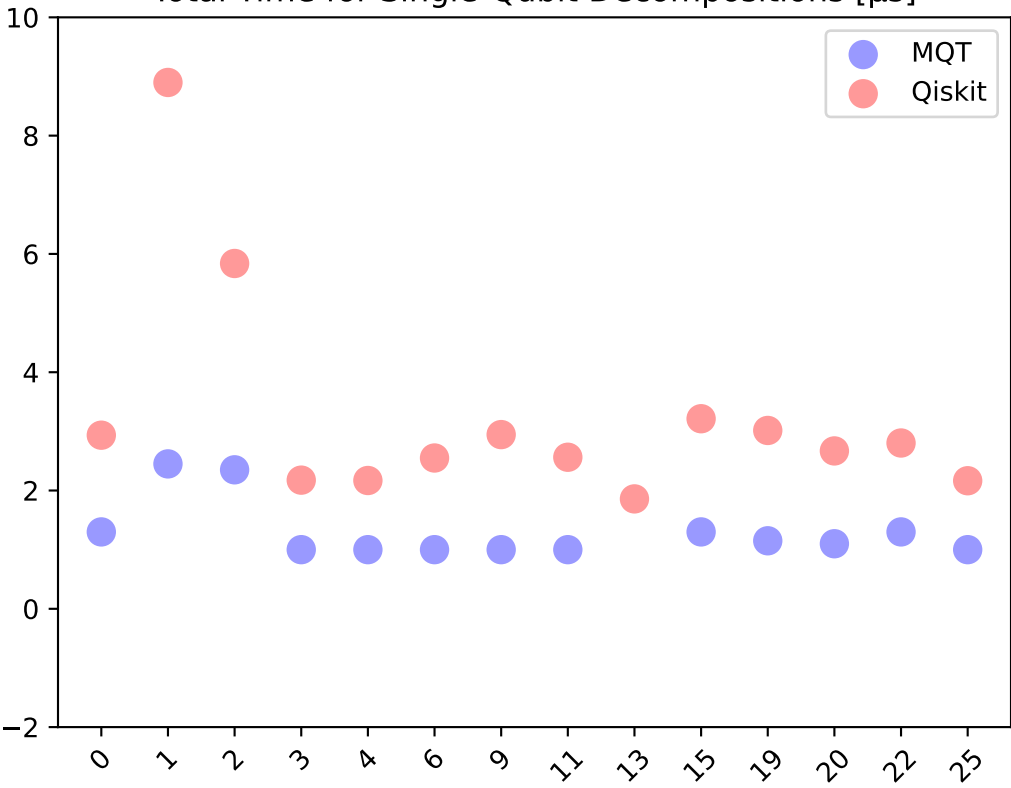
Total Time for Single-Qubit Decompositions [ \mu s]
