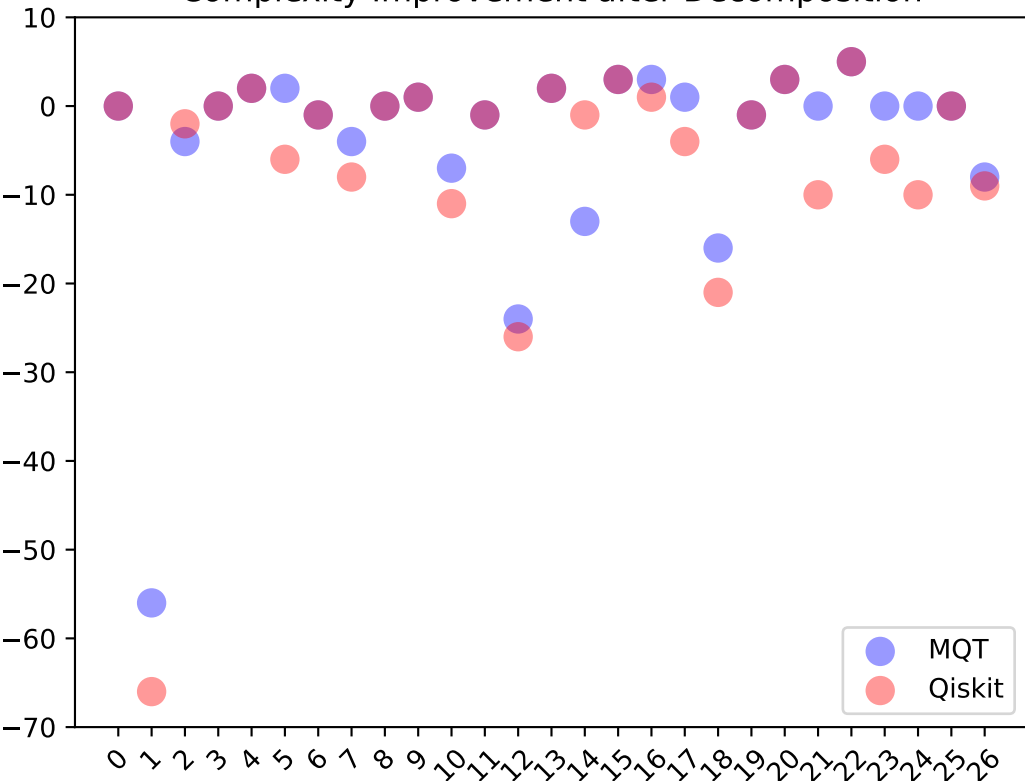
Complexity Improvement after Decomposition
