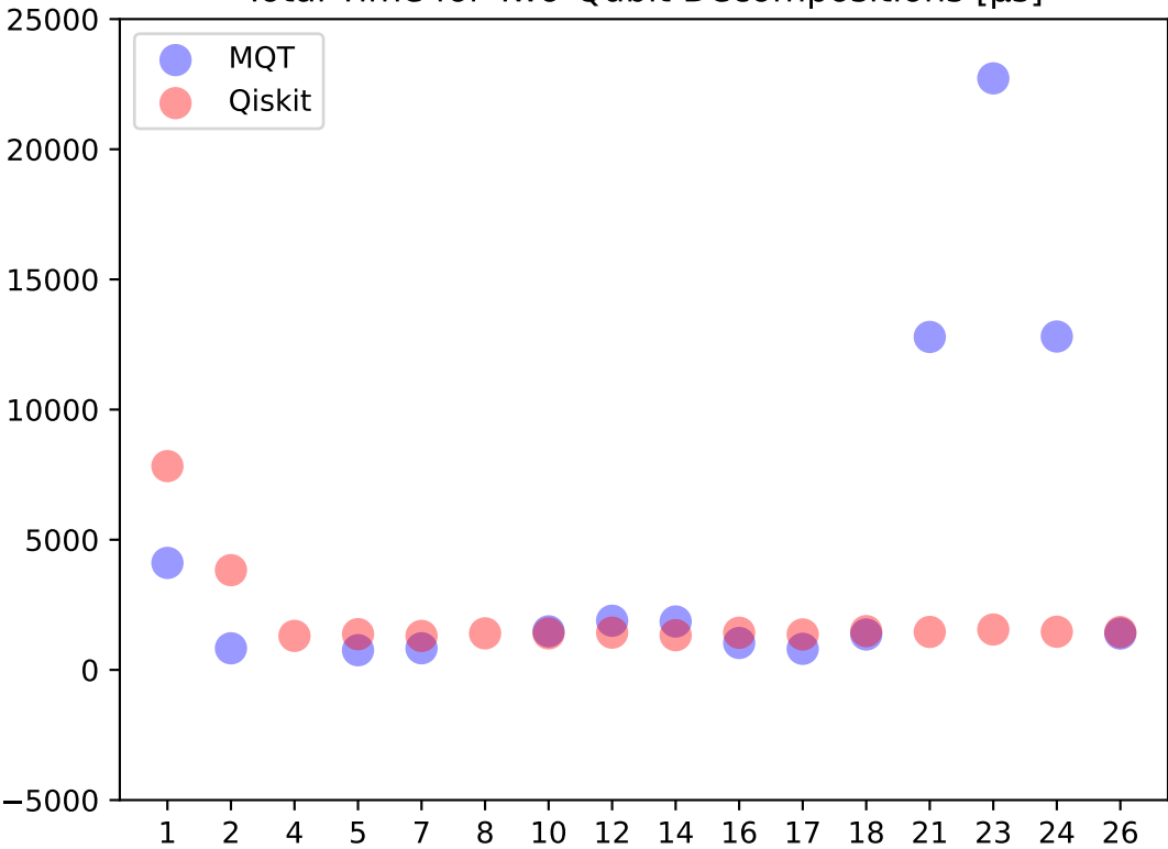
Total Time for Two-Qubit Decompositions [ \mu\text{s} ]
