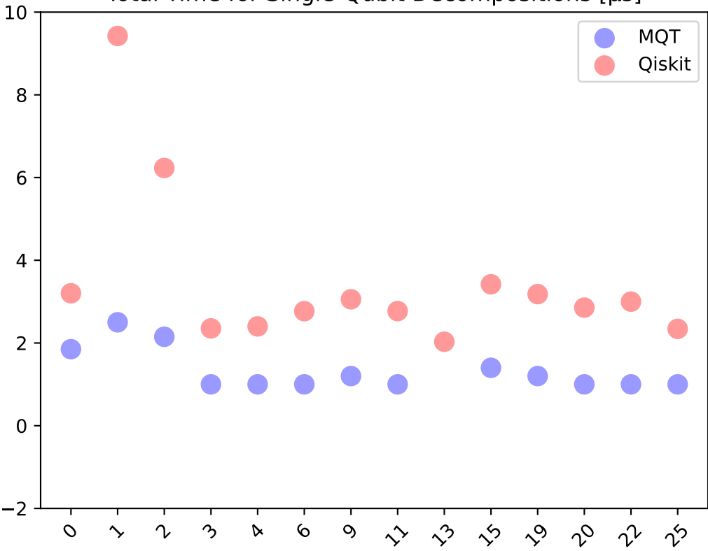
Total Time for Single-Qubit Decompositions [ \mu\text{s} ]
