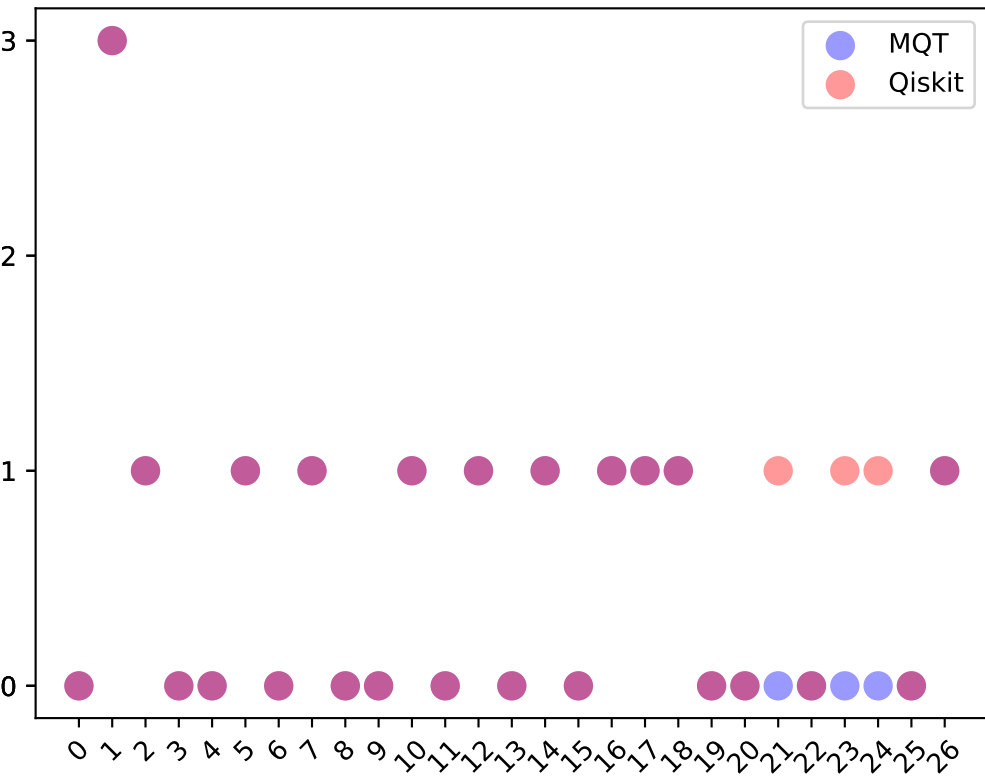
Number of Successful Two-Qubit Decompositions
