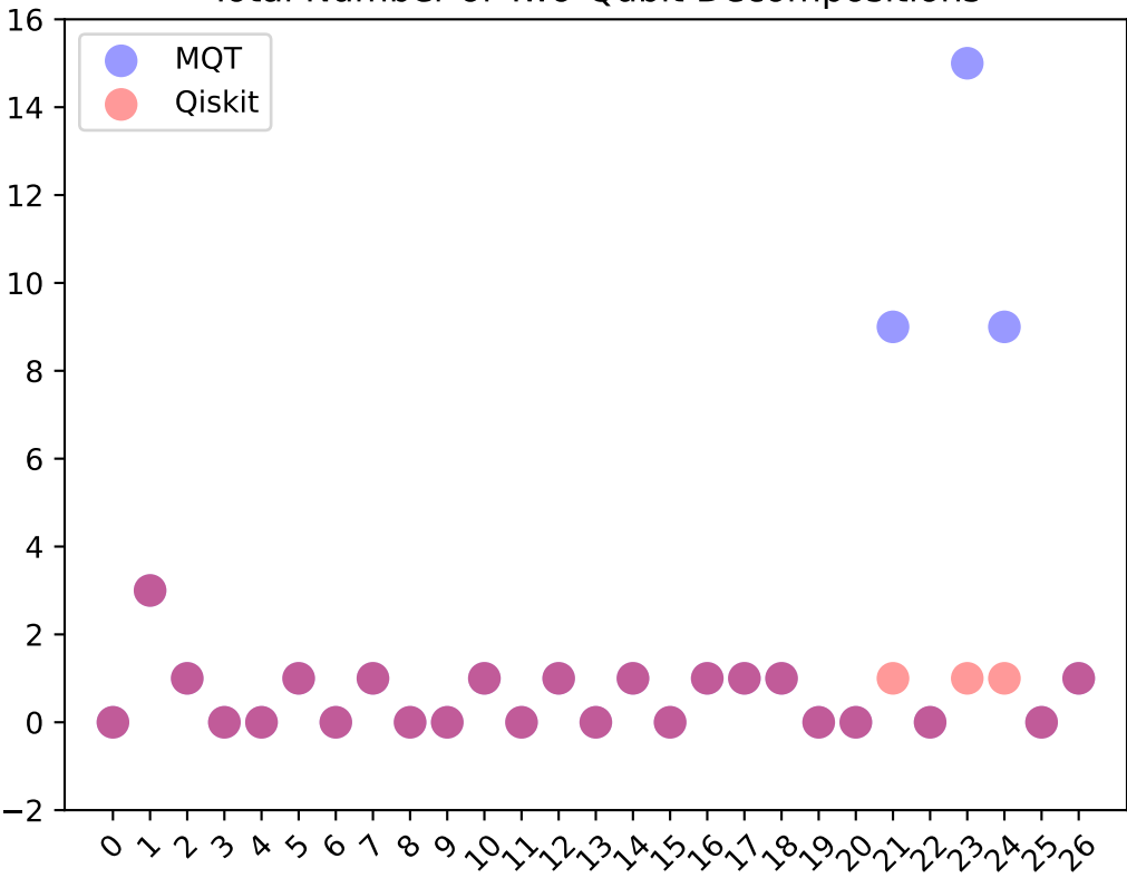
Total Number of Two-Qubit Decompositions
