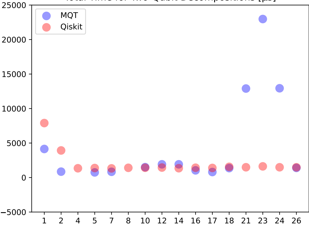
Total Time for Two-Qubit Decompositions [ \mu s]
