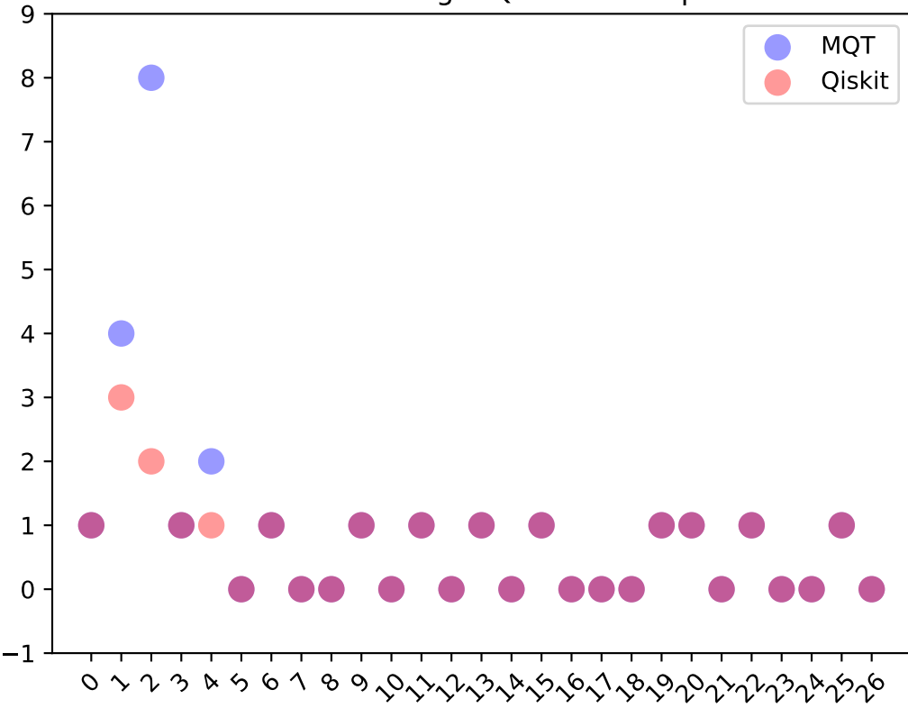
Total Number of Single-Qubit Decompositions
