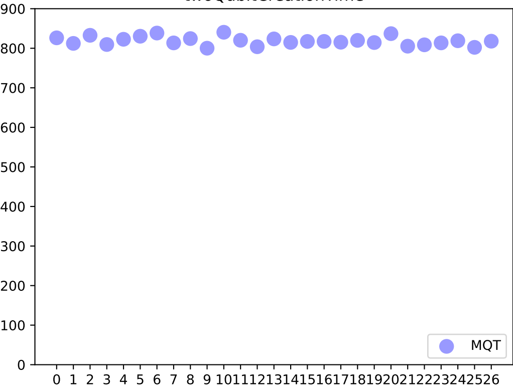
twoQubitCreationTime
