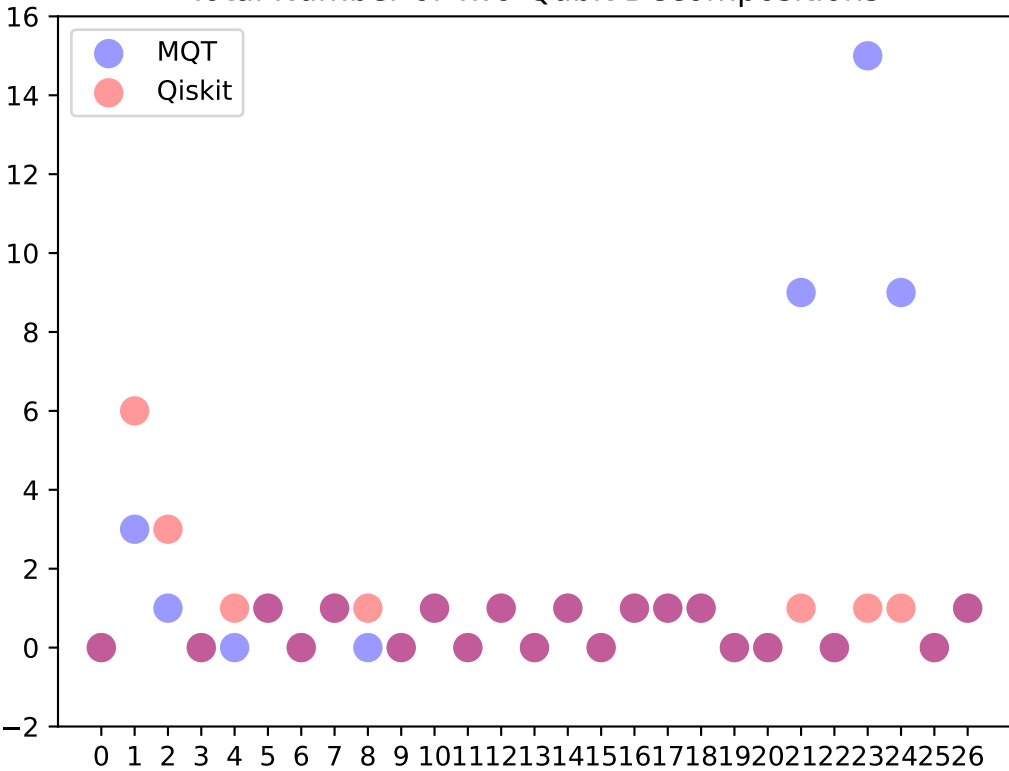
Total Number of Two-Qubit Decompositions
