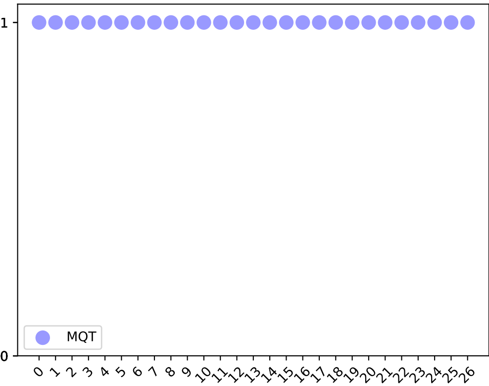
numberOfTwoQubitCreations
