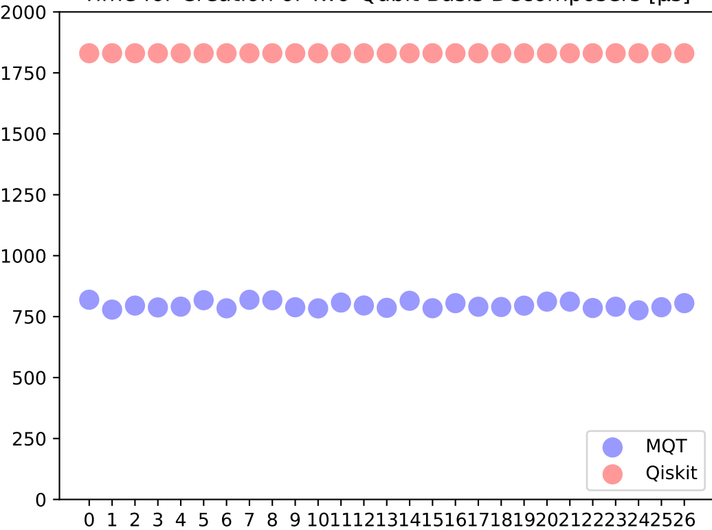
Time for Creation of Two-Qubit Basis Decomposers [ \mu s]
