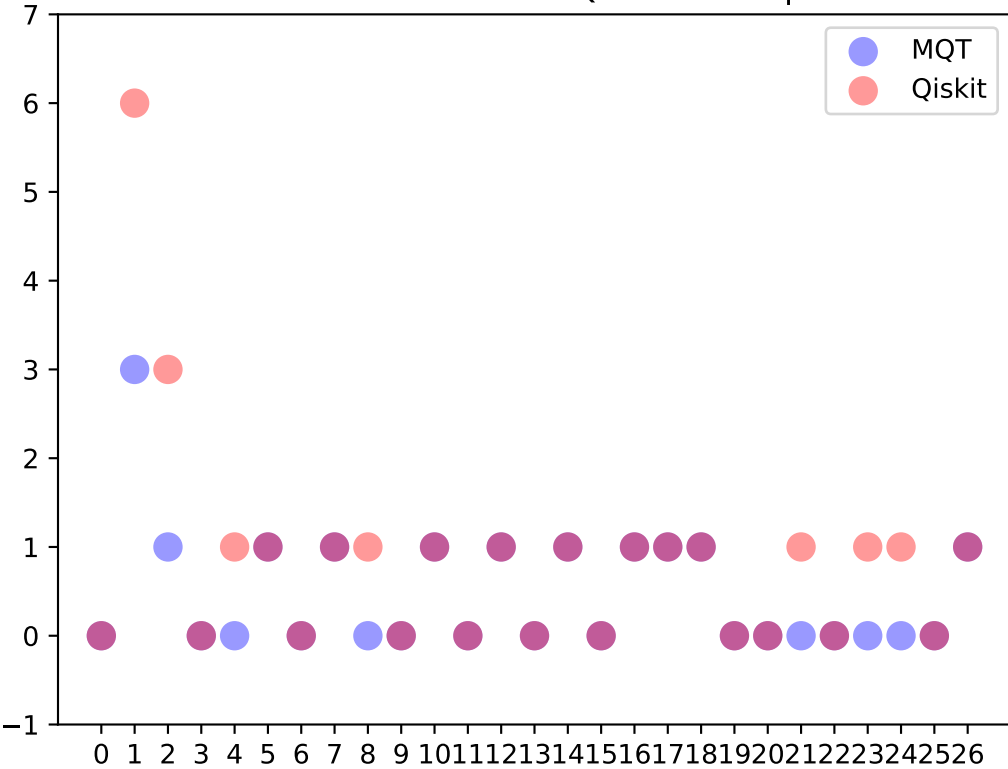
Number of Successful Two-Qubit Decompositions
