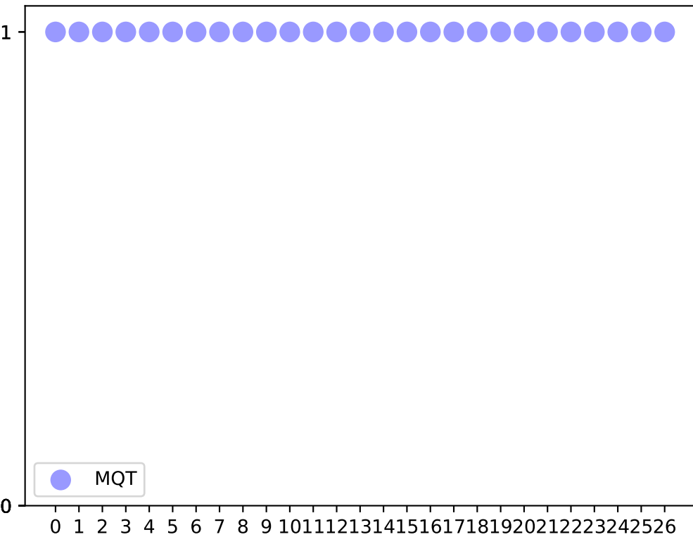
numberOfTwoQubitCreations
