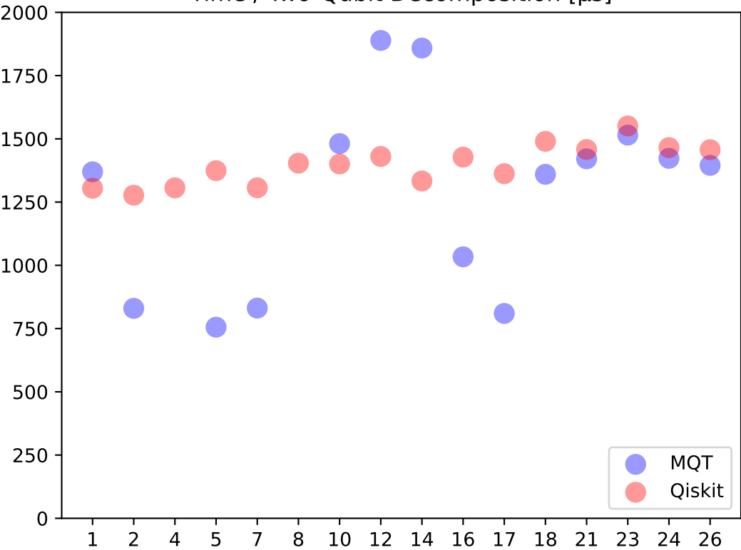
Time / Two-Qubit Decomposition [ \mu s]
