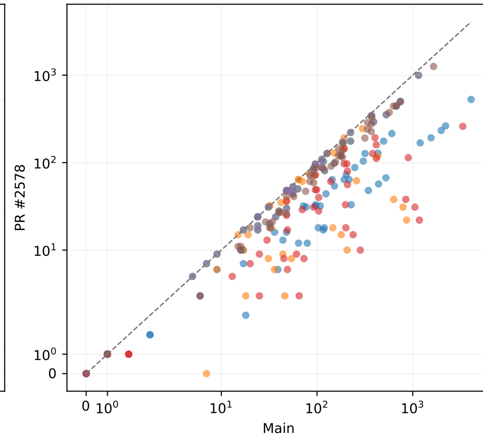
Large · One-qubit gates excluding RZ
