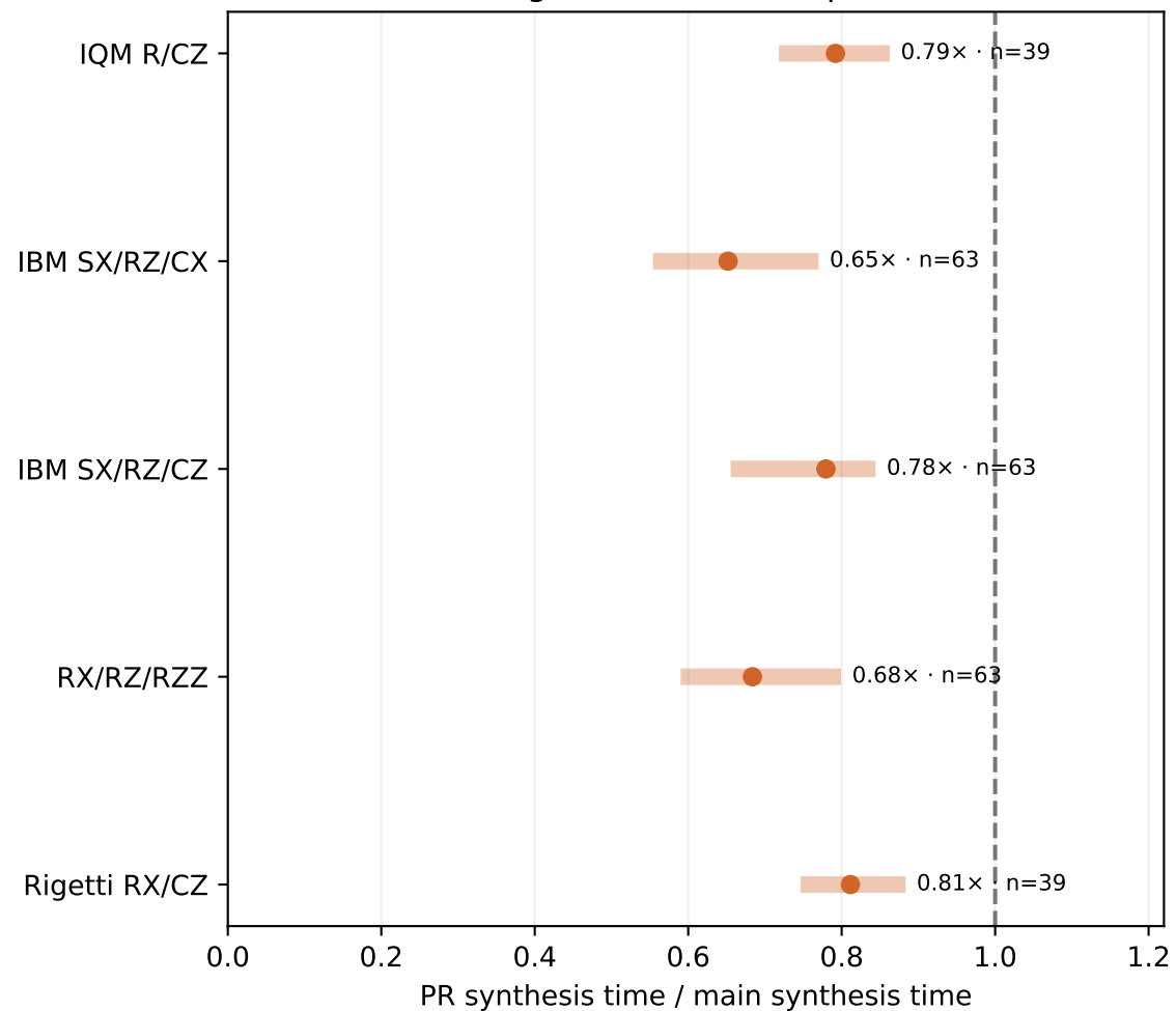
Large suite: 24-156 qubits
