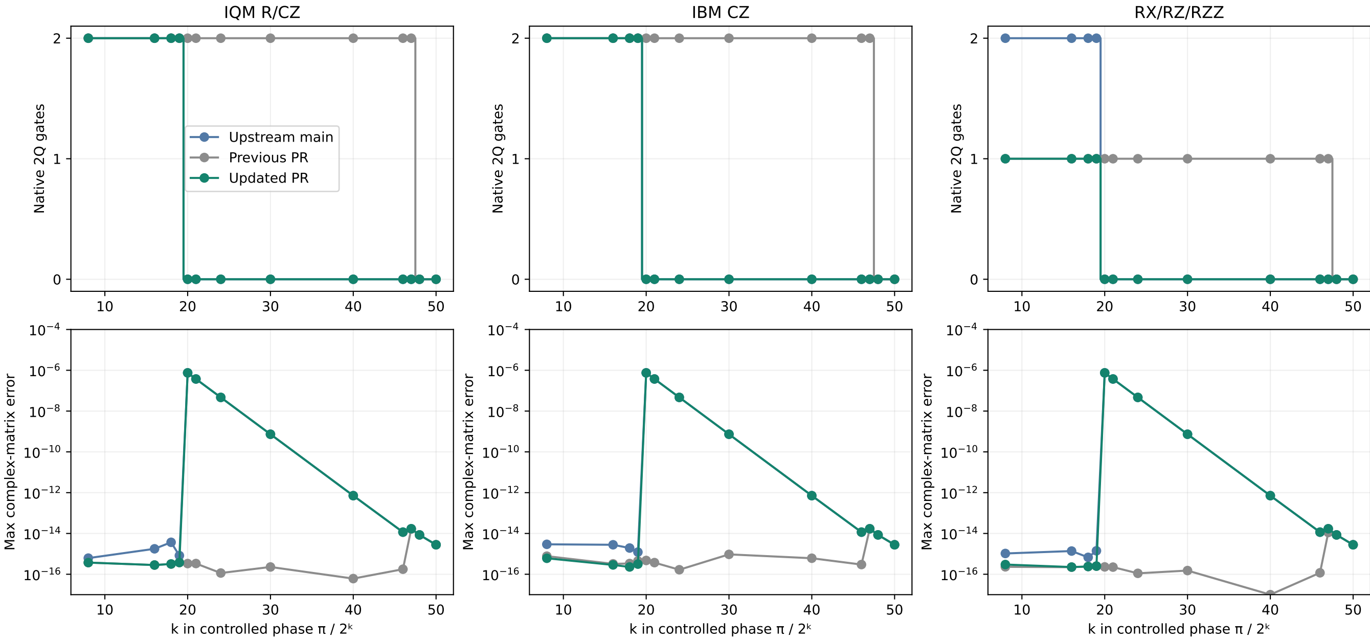
Direct Pauli and numeric Weyl synthesis now share the small-angle policy Two-qubit probe: exact matrix comparison including phase; errors below 1e-17 shown at plotting floor
