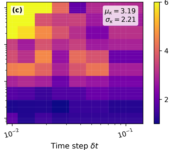
Sampling Inflation
