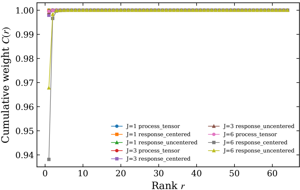
Cut c = 2
