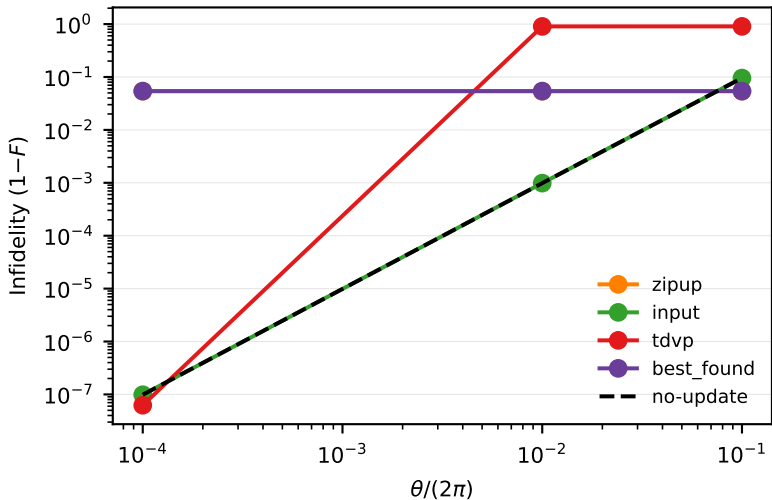
Variational-MPO initializers ( \chi_{\max} = 8 , 4 sweeps)
