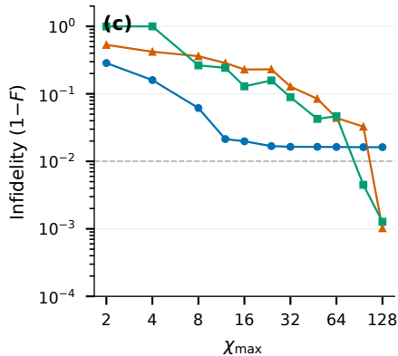
4×4 Heisenberg, one Trotter step
