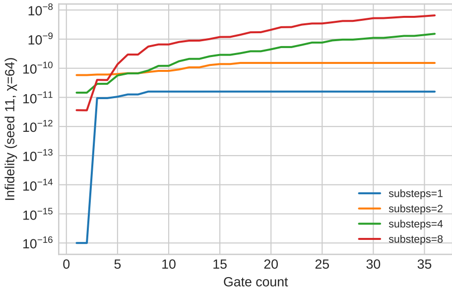
TDVP substep diagnostic (v2 database)
