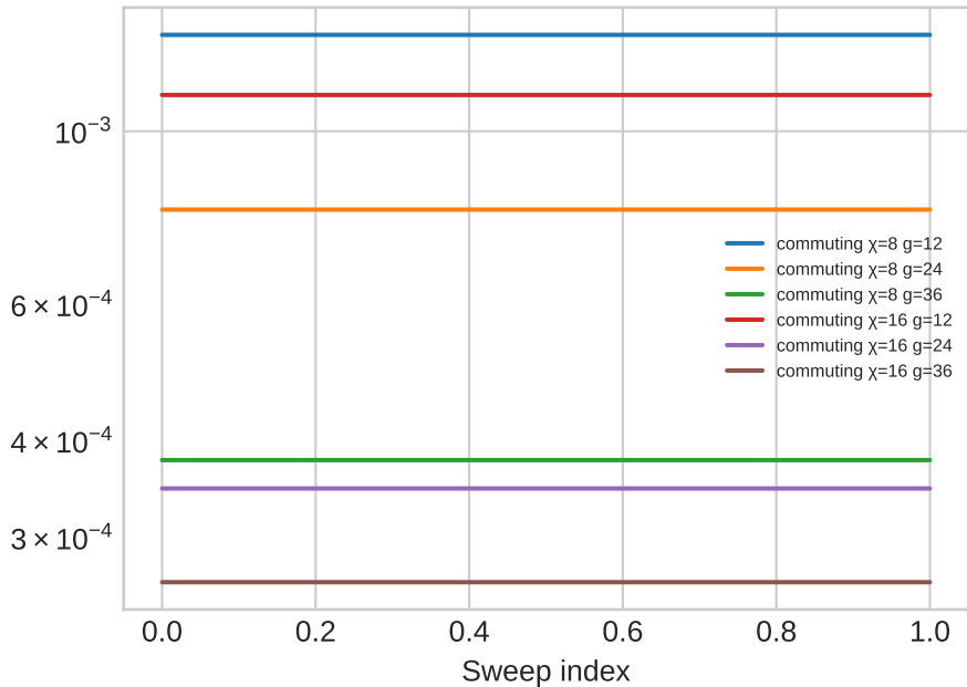
Variational objective
