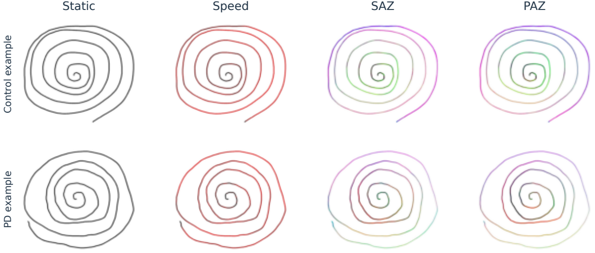
Figure 2: Building a pseudodynamic image from the same spiral trace. Rows show one control and one PD example, selected by a fixed identifier rule without reference to prediction quality. Columns move from static geometry to speed alone and two RGB triplets. The trajectory is unchanged; colour describes within-recording variation.
