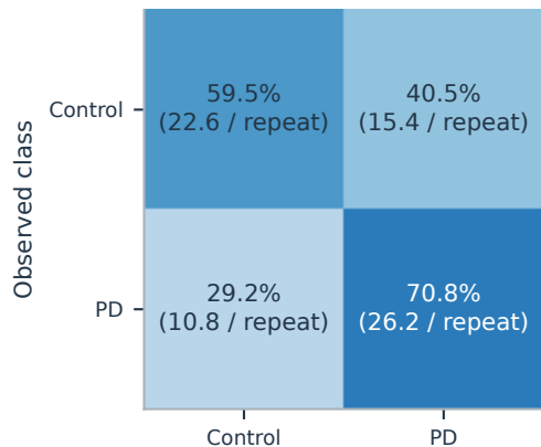
Logistic regression
