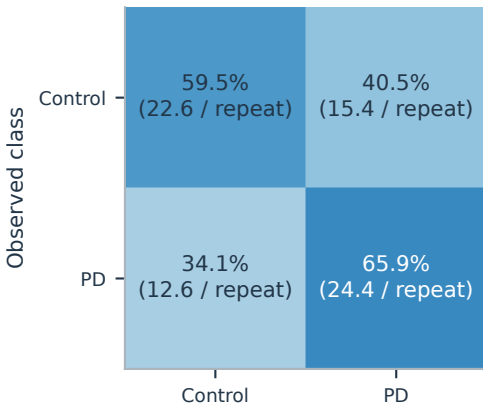
Random forest
