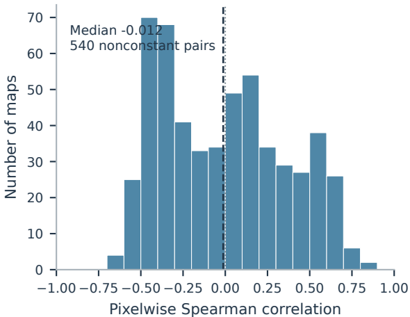
Grad-CAM vs occlusion
