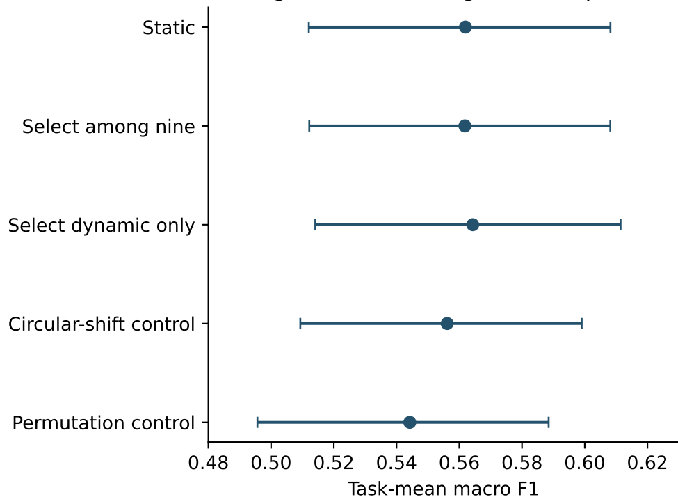
All eight tasks: training-selected policies
