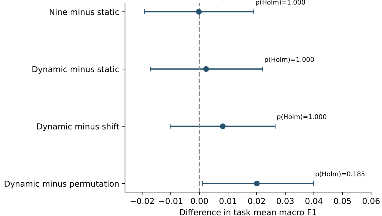
Four paired contrasts
