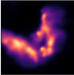
forecast (CasCast backbone) observed, max 16^2 , \geq 219
