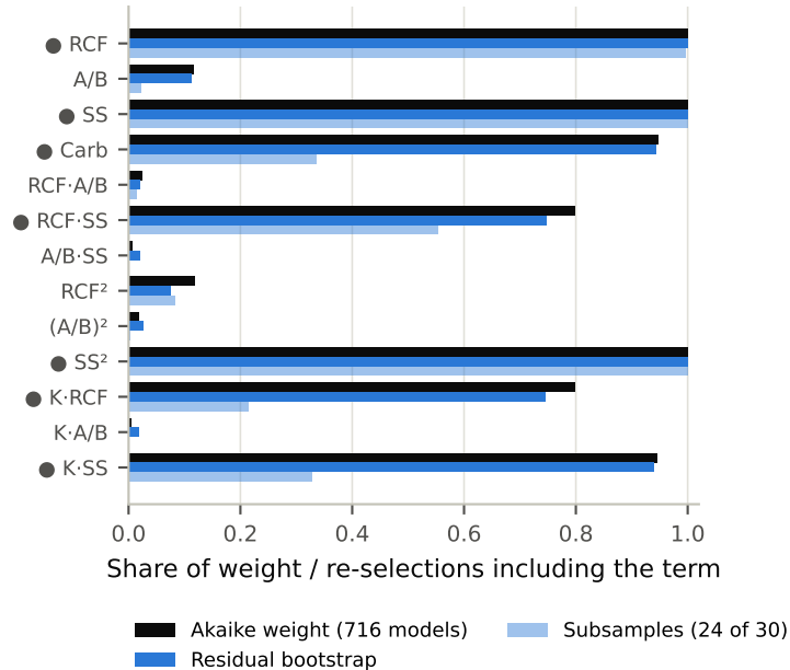
b 7-day model: term support (● = selected)
