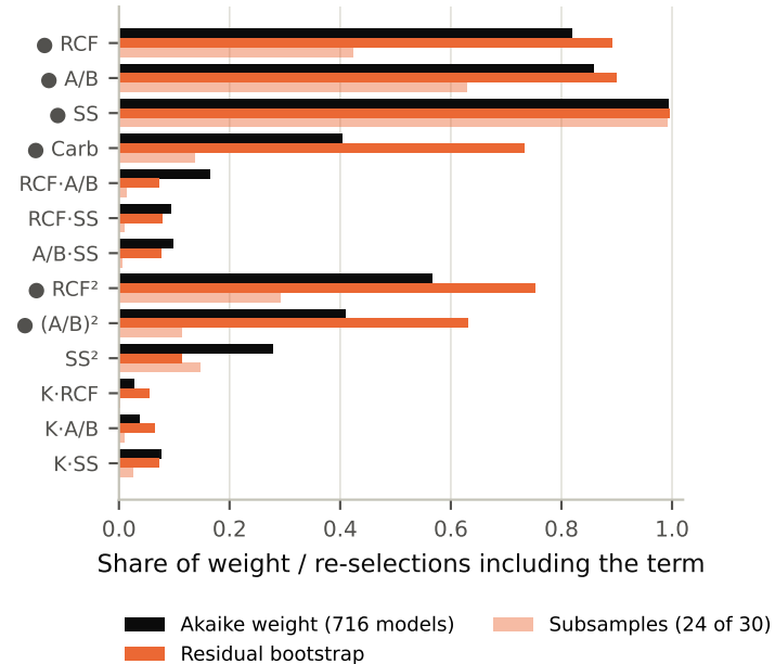
c 28-day model: term support (● = selected)
