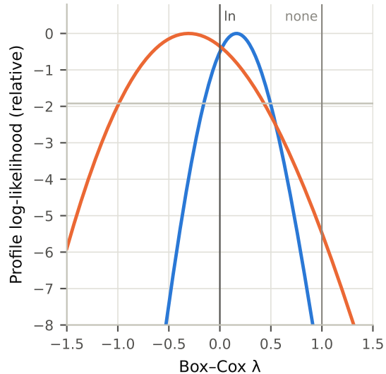
a Response scale (selected models)
