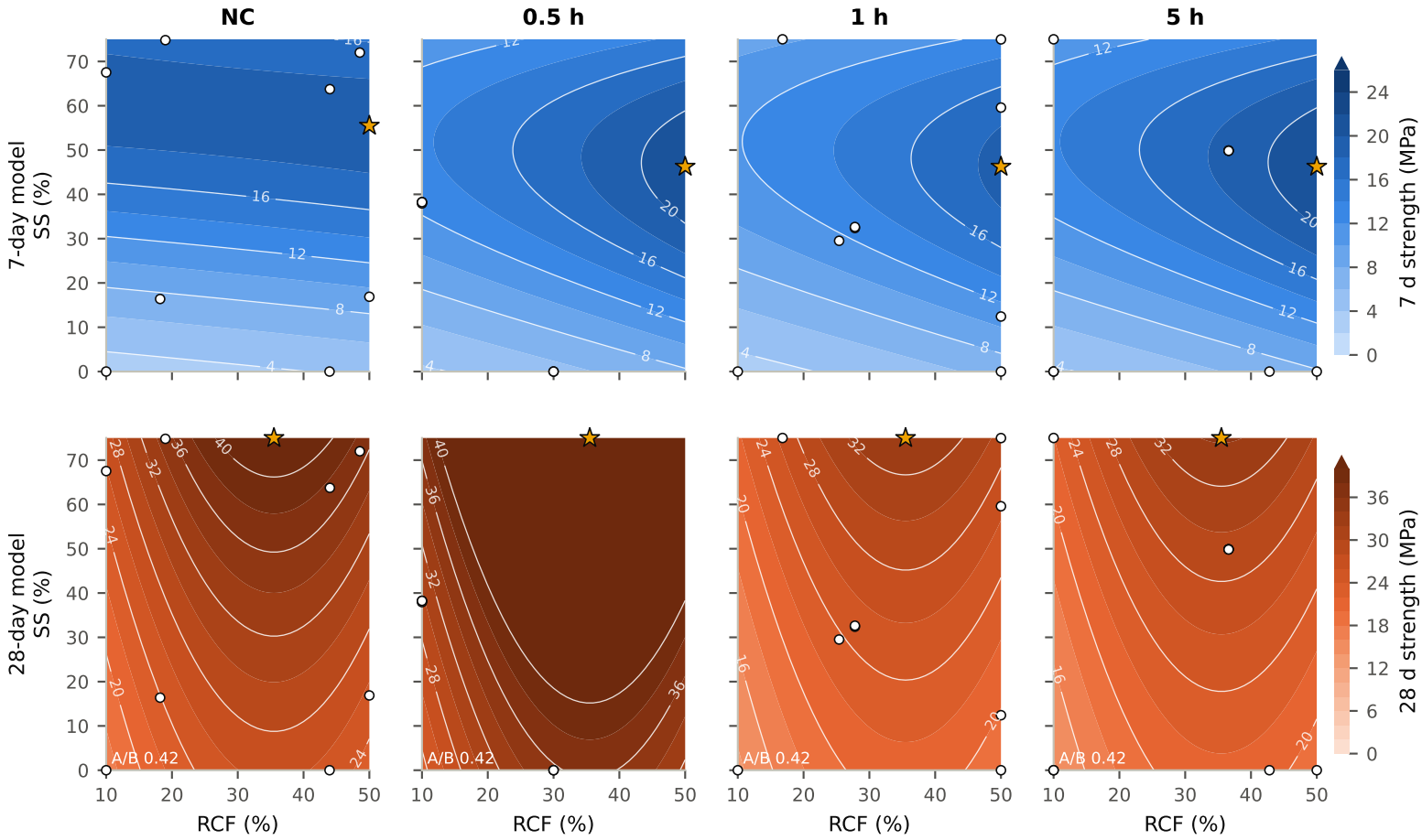
Median predicted strength over RCF \times SS from each model (own colour scale per age). \circ runs at that level, \star maximum
