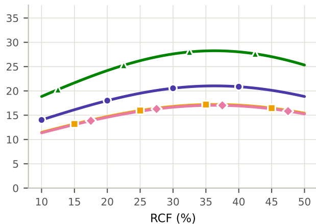
d 28 d — strength vs RCF (SS 37.5 %, A/B 0.45)
