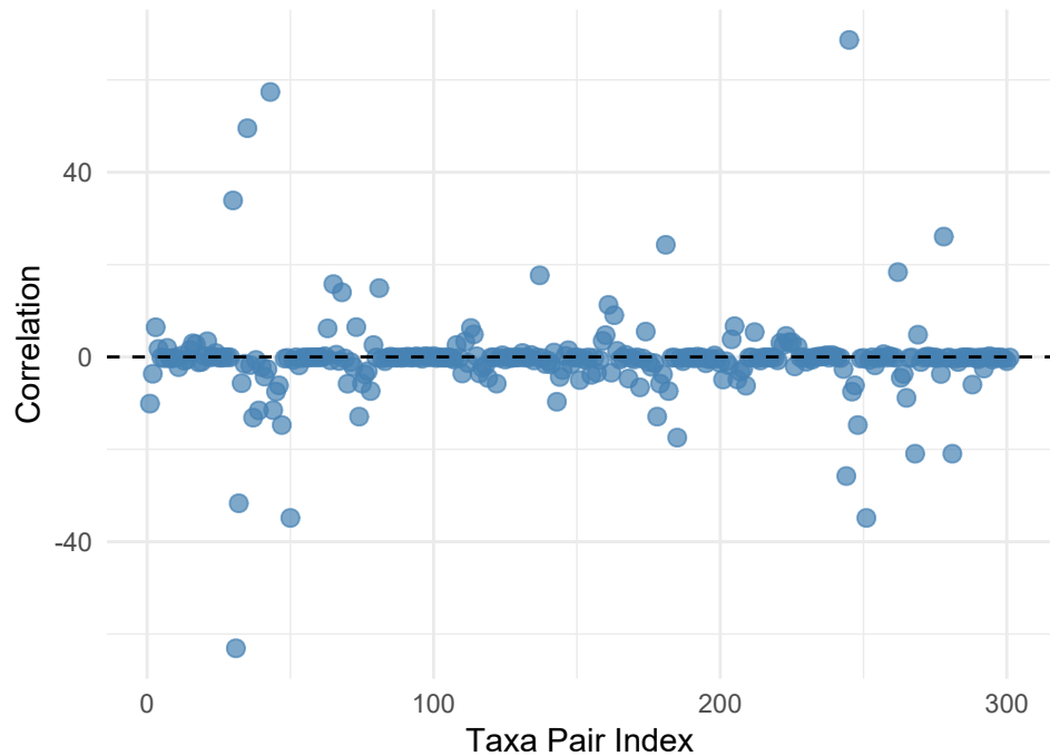
Original \hat{\Gamma} ( |\text{correlation}| > 0.05 )
