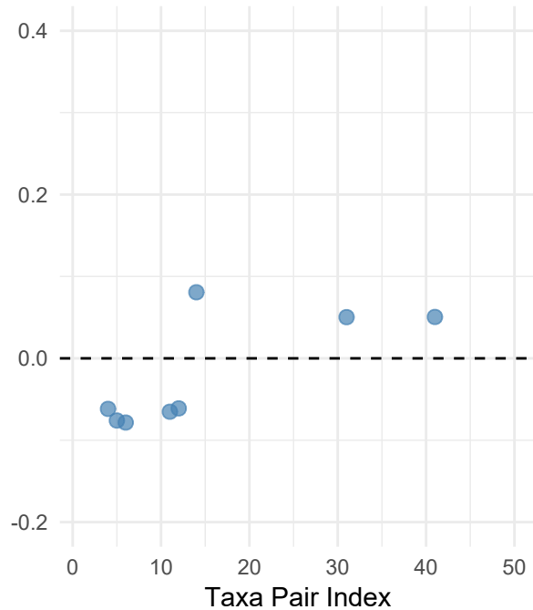
Empirical \hat{\rho}^* ( |\text{correlation}| > 0.05 )
