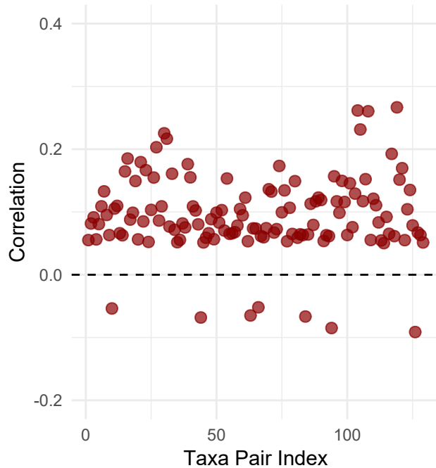
\hat{\tau}_{\text{ZI}}^* ( |\text{correlation}| > 0.05 )
