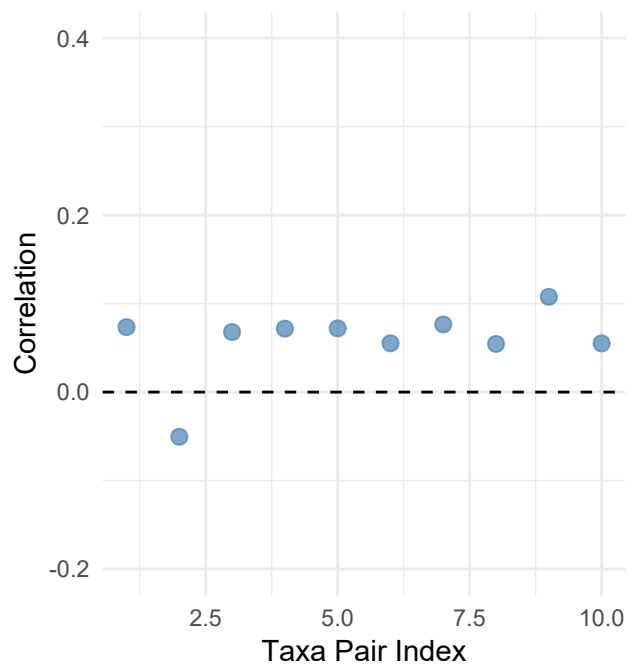
\hat{\tau}_{\text{Emp}}^* ( |\text{correlation}| > 0.05 )
