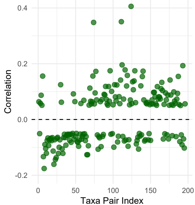
\hat{\tau}_{\text{Org}}^* ( |\text{correlation}| > 0.05 )
