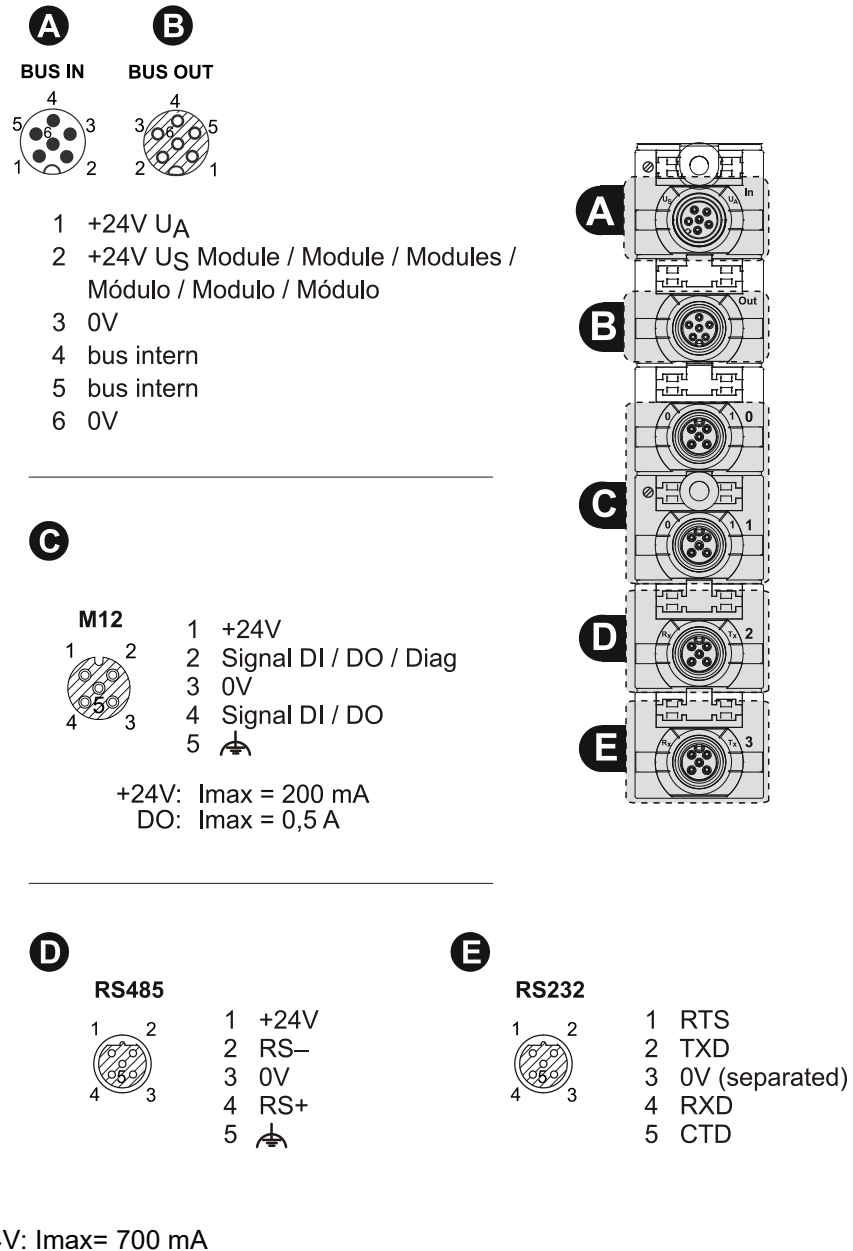
Fig. 67: Connection overview Cube67+ DIO4 RS232/485 E 4xM12 – Art.-No. 56761
