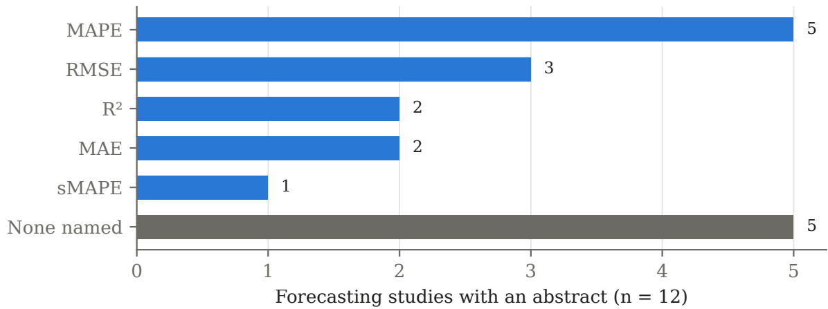
Figure 7: Accuracy measures named in the abstracts of forecasting studies. A study can name several measures.
