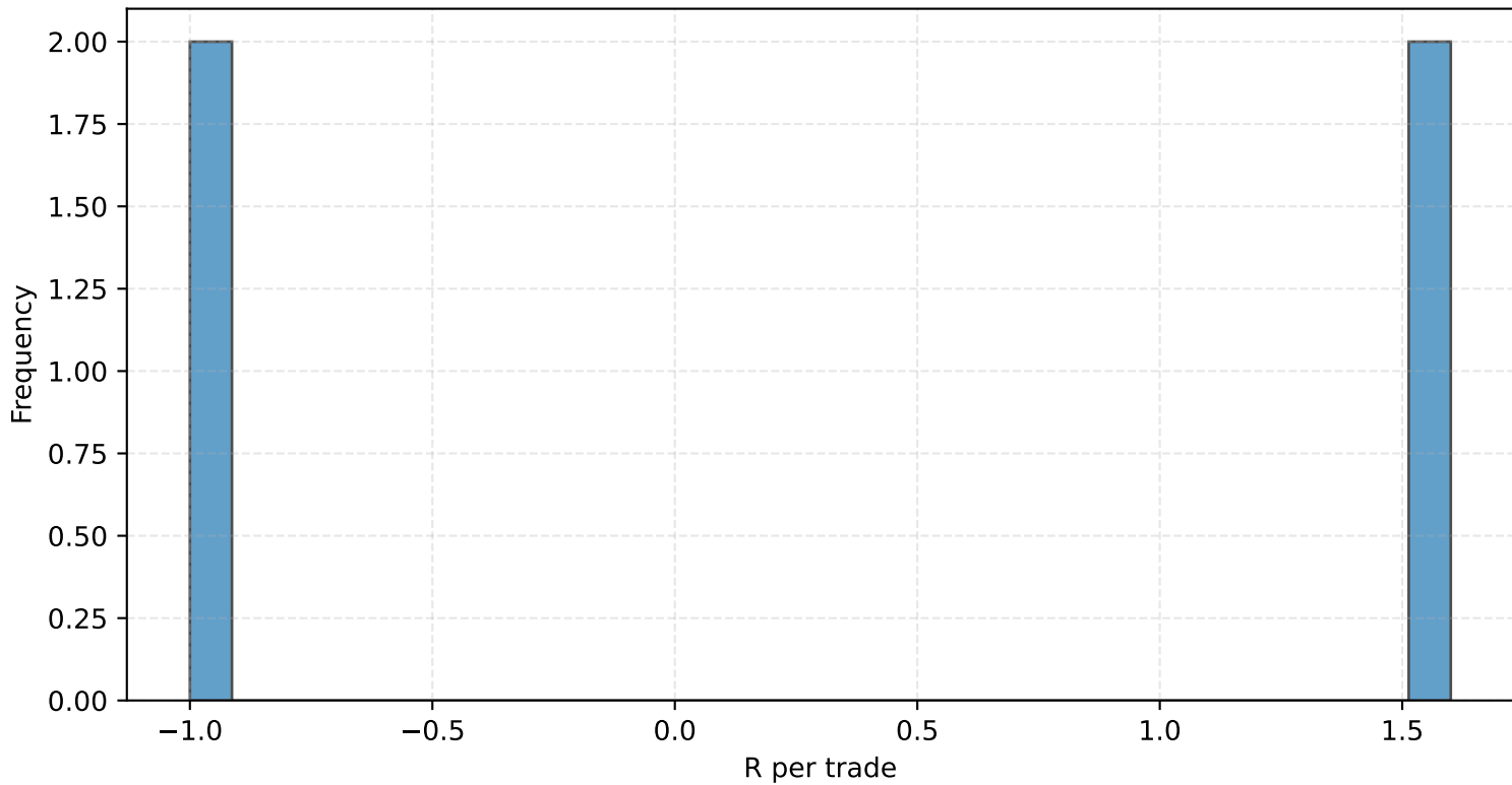
Distribution of R per Trade
