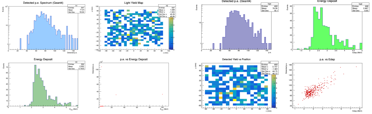
Figure 2: Combined Geant4 results from 500-event run + position scan of the improved model (processed with ROOT): (left) 4-panel overview (PE spectrum, Edep, yield map, correlation); (right) updated clean analysis plots.
