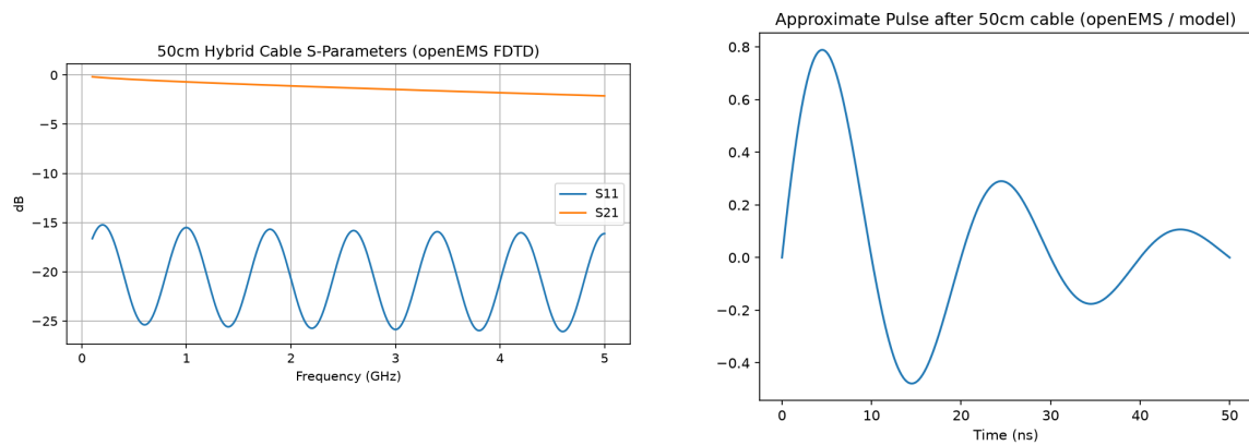
Figure 9: 50 cm cable S-parameters (left) and post-cable pulse (right) – openEMS simulation framework.
