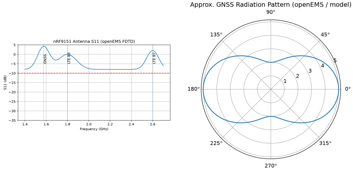
Figure 8: nRF9151 antenna S11 (left) and approximate radiation pattern (right) from openEMS-enabled simulation.
