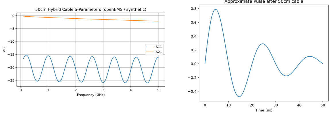
Figure 8: 50 cm cable S-parameters (left) and post-cable pulse (right).
