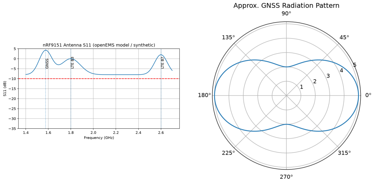
Figure 7: nRF9151 antenna S11 (left) and approximate radiation pattern (right) from openEMS model.
