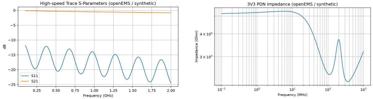
Figure 9: High-speed trace S-params (left) and 3V3 PDN impedance (right).
