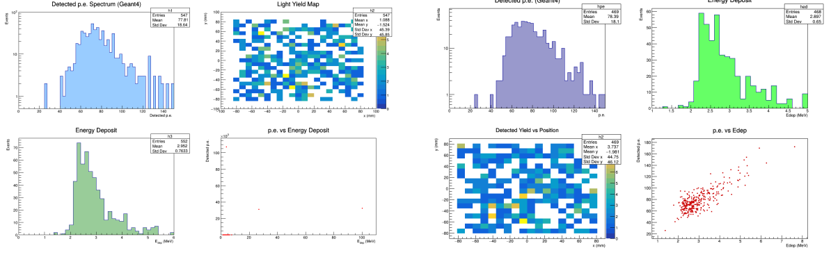
Figure 1: Combined Geant4 results from 500-event run + position scan of the improved model (processed with ROOT): (left) 4-panel overview (PE spectrum, Edep, yield map, correlation); (right) updated clean analysis plots.
