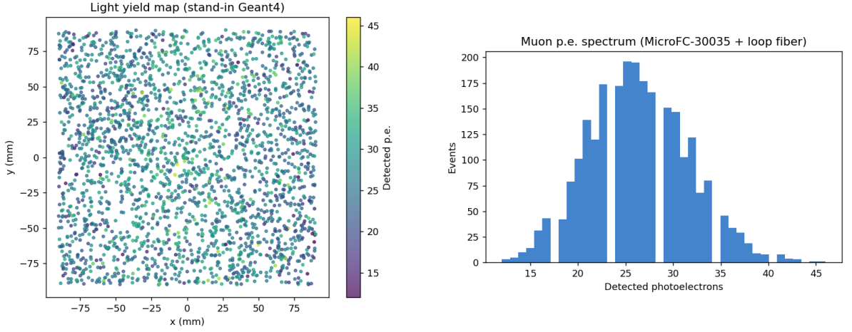
Figure 2: Light yield map (left) and photoelectron spectrum (right) from the Geant4 optical simulation.
