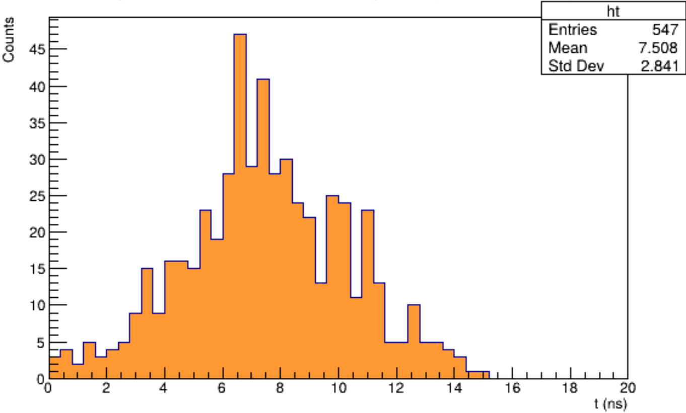
Optical Photon Arrival Time Spread (Geant4 model)
