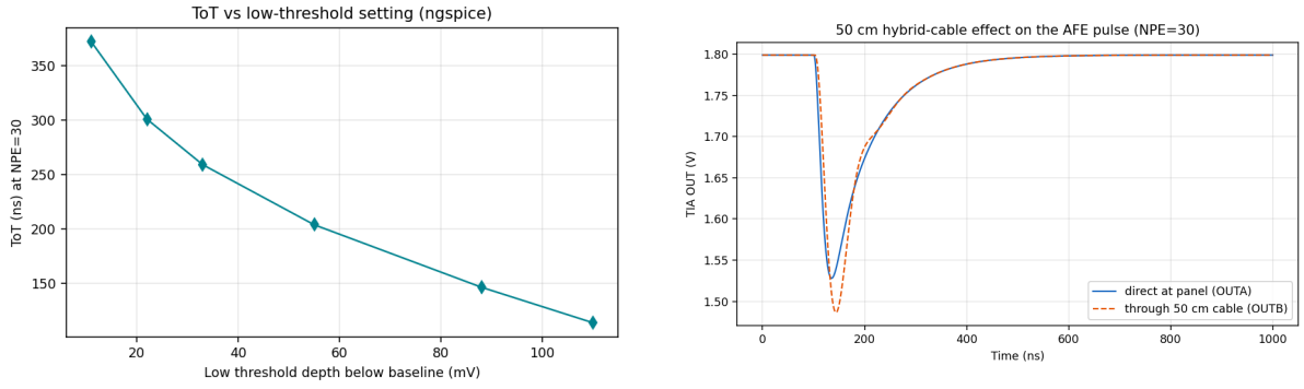
Figure 6: Left: Threshold scan at NPE=30 showing ToT sensitivity. Right: Cable comparison (direct vs 50 cm) impact on pulse fidelity.
