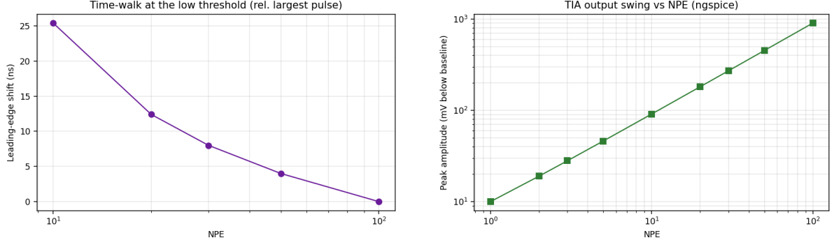
Figure 5: Left: Leading-edge time-walk vs NPE. Right: Peak amplitude (mV) vs NPE from ngspice AFE sweeps.
