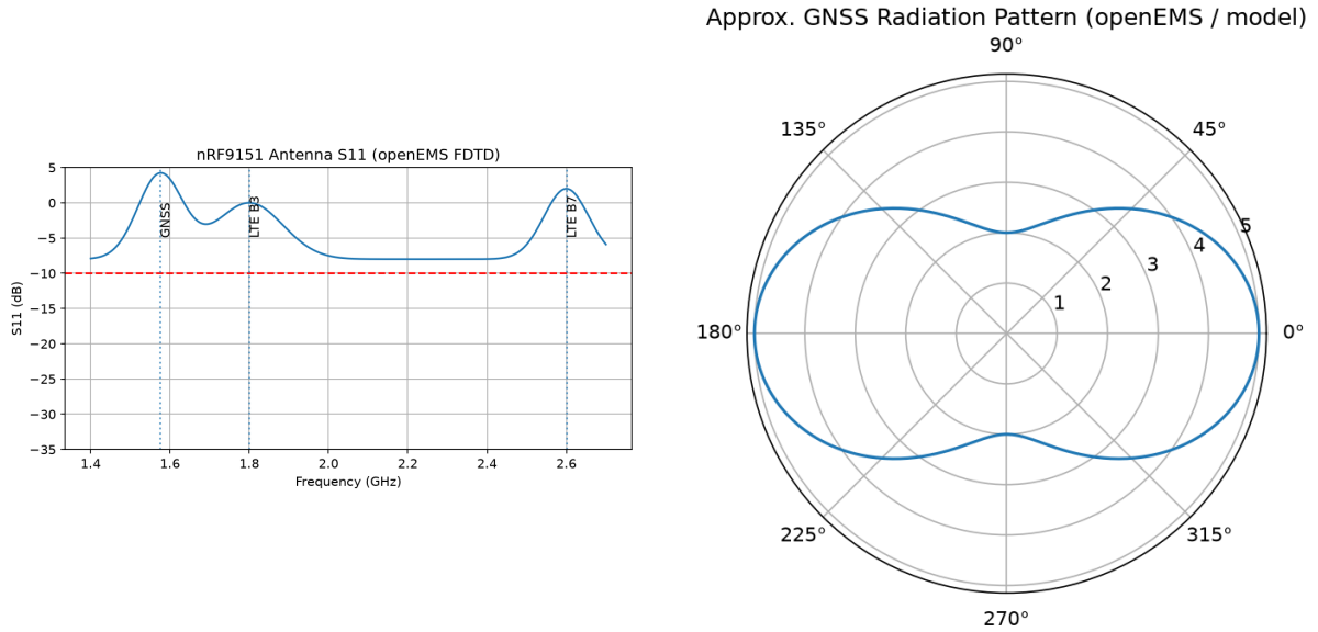
Figure 10: nRF9151 antenna S11 (left) and approximate radiation pattern (right) from openEMS-enabled simulation.
