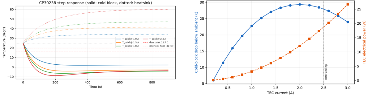
Figure 8: CP30238 step responses (left) and steady-state sweep (right). 1.5–1.8 A gives \sim 25 – 29 K cooling; Joule heating limits gains above \sim 2 A. Electrical power per channel \sim 7 – 10 W at useful operating point.
