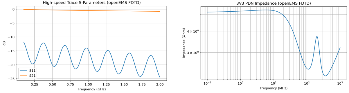
Figure 12: High-speed trace S-params (left) and 3V3 PDN impedance (right) from openEMS simulations.
