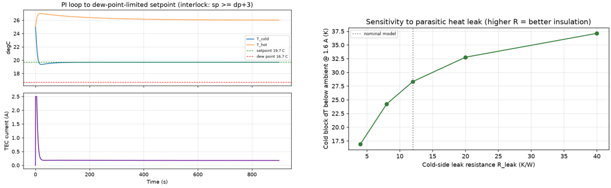
Figure 9: Left: Closed-loop PI response to a dew-point-limited setpoint. Right: sensitivity of achievable \Delta T to cold-cavity insulation ( R_{leak} ). Good sealing is essential.
