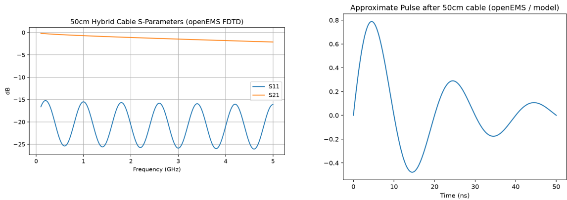
Figure 11: 50 cm cable S-parameters (left) and post-cable pulse (right) – openEMS simulation framework.
