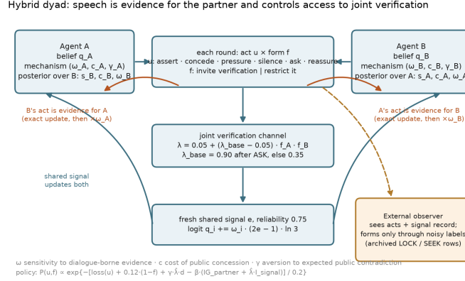
Fig. 1. Hybrid dyad. Each round both agents choose an act and a form; the joint verification channel delivers a shared signal only when both invite; the partner’s act is evidence through a level-0 model of the partner; an external observer sees acts and signals and forms only through noisy Part I labels.
