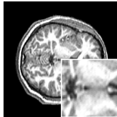
CycleGAN
