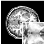
CycleGAN
