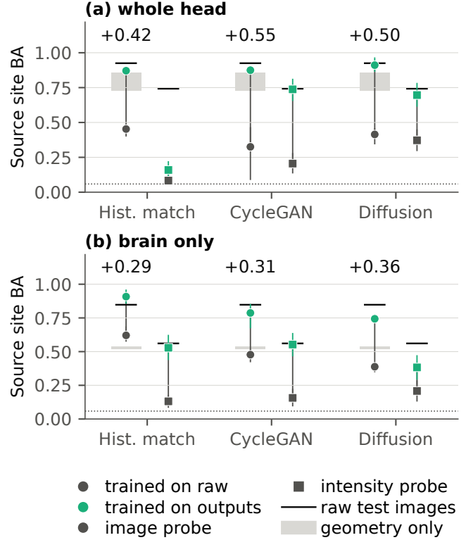
Fig. 1. Probes trained on raw slices (grey) or on a method's outputs (aqua), tested on that method's outputs (diffusion: second draw), on (a) whole heads and (b) brain-only slices: image probes (circles, mean and range over 3 seeds) and intensity-histogram probes (squares, 95% interval). Numbers: paired difference in three-seed mean BA between output- and raw-trained image probes. Black bar: raw-trained probe on raw test slices. Grey: image probes given only head silhouettes or brain masks. Dotted line: uniform chance.
