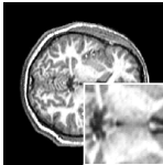
CycleGAN
