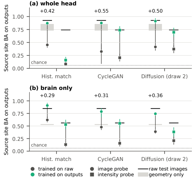
Fig. 1. Probes trained on raw slices (grey) or a method’s outputs (aqua), tested on its outputs (diffusion: draw 2), on (a) whole heads and (b) brains: image probes (circles, mean and range over 3 seeds) and intensity-histogram probes (squares, 95% interval). Numbers: paired output minus raw-trained difference. Black bar: raw-trained probe on raw slices. Grey: silhouette or brain-mask probes.
