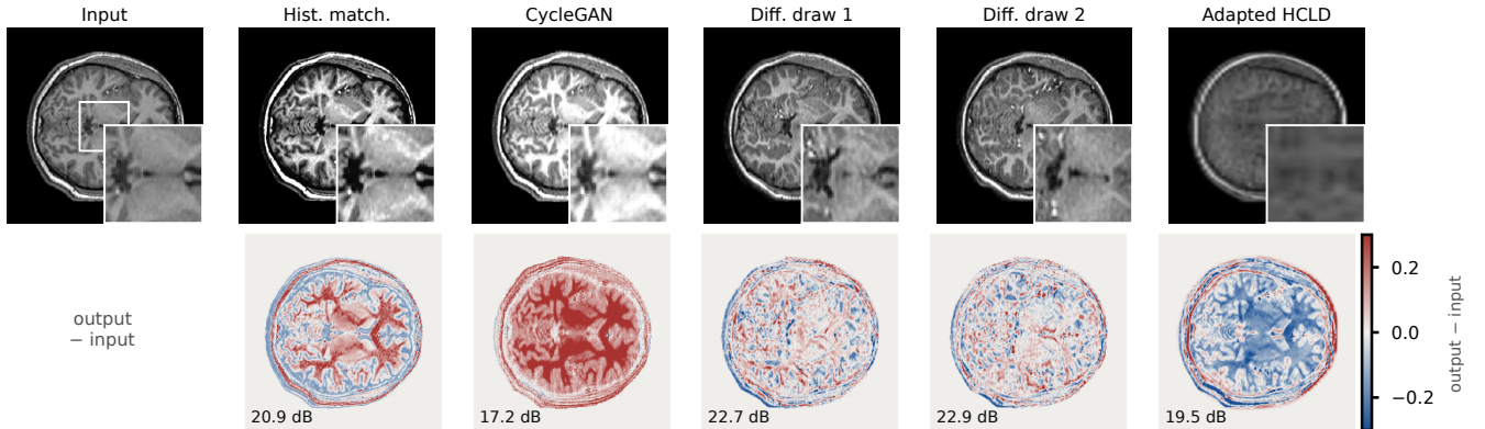
Fig. 2. Source subject with median PSNR over nine outputs (all but DLEST-style 1500); insets: 2\times zoom of the box. Bottom: output – input, with PSNR. The adapted HCLD output loses anatomy; diffusion adds texture that differs between draws.
