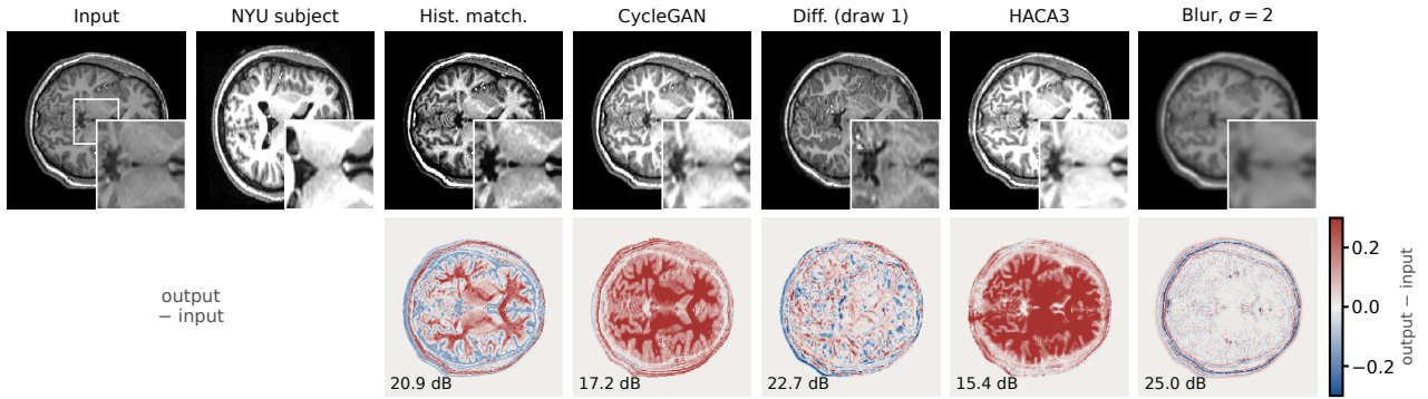
Fig. 2. One source subject (median PSNR) and an NYU subject with a similar slice, in the input’s intensity window, with 2 \times zoomed insets. Bottom: output minus input, with PSNR. The blur has the highest PSNR of the outputs shown.
