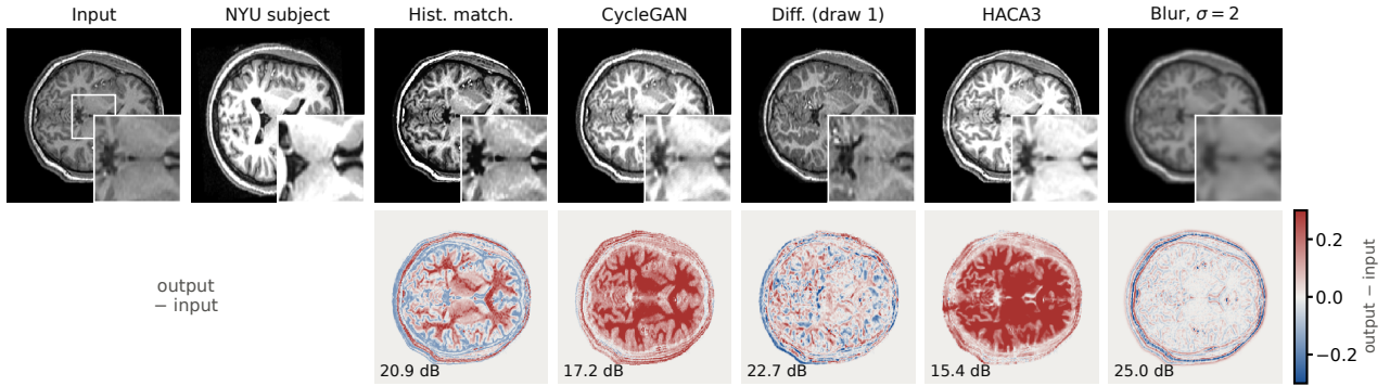
Fig. 2. One source subject (median PSNR) and an NYU subject with a similar slice, in the input’s intensity window, with 2\times zoomed insets. Bottom: output minus input, with PSNR. The blur has the highest PSNR of the outputs shown.
