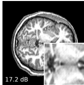
CycleGAN
