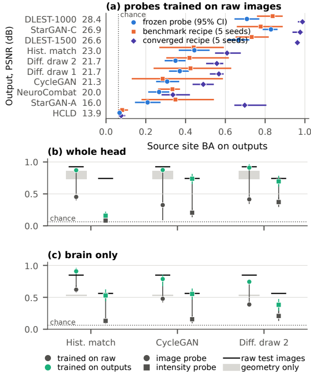
Fig. 2. (a) Source site BA of each output, ordered by PSNR; retrained probes show the mean and range over five seeds. (b, c) Probes trained on raw slices (grey) or on a method’s outputs (aqua), tested on that method’s outputs (diffusion: second draw), on whole heads and on brain-only slices: image probes (circles, mean and range over 3 seeds) and intensity-histogram probes (squares, 95% interval). Black bar: raw-trained probe on raw test slices. Grey: image probes given only head silhouettes or brain masks.
