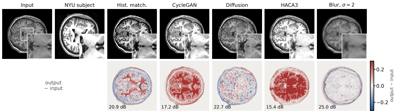
Fig. 2. Median-PSNR source subject and an axial NYU slice with similar head outline and anatomy, in the input’s window; insets: 2\times zoom of the box. Bottom: output – input with PSNR. HACA3 shifts contrast; blur has the highest PSNR.
