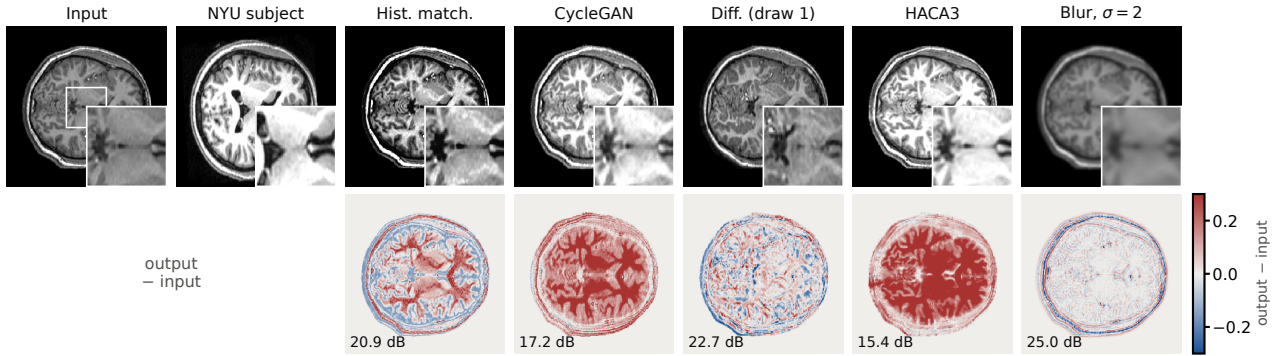
Fig. 2. A typical source subject (median PSNR across outputs) and an NYU test subject whose slice best matches the input’s head outline and anatomy, on the input’s brightness scale; insets zoom 2\times into the box. Bottom: output – input, with PSNR.
