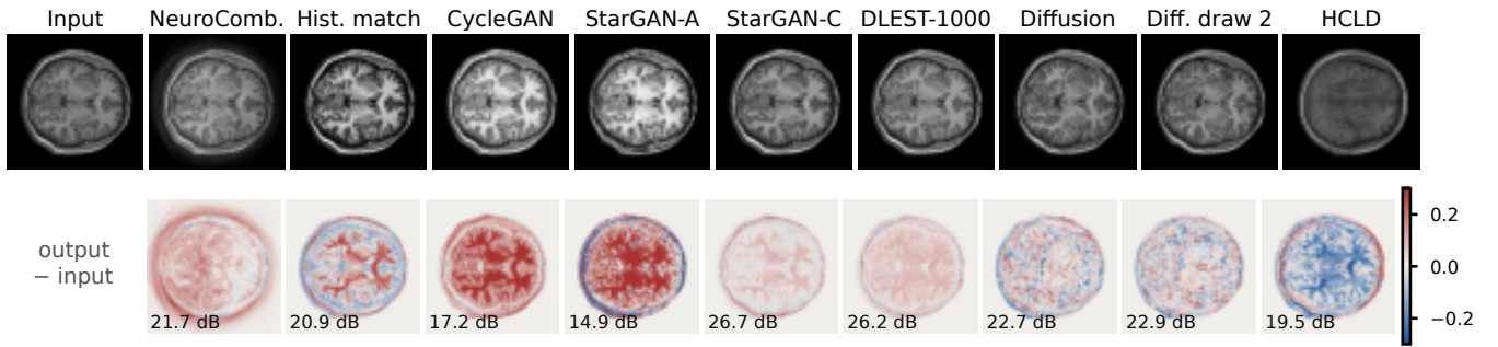
Fig. 2. One source test subject (chosen as the median of PSNR averaged over outputs). Bottom: output minus input, with PSNR. HCLD loses anatomical detail; diffusion adds texture that differs between draws.
